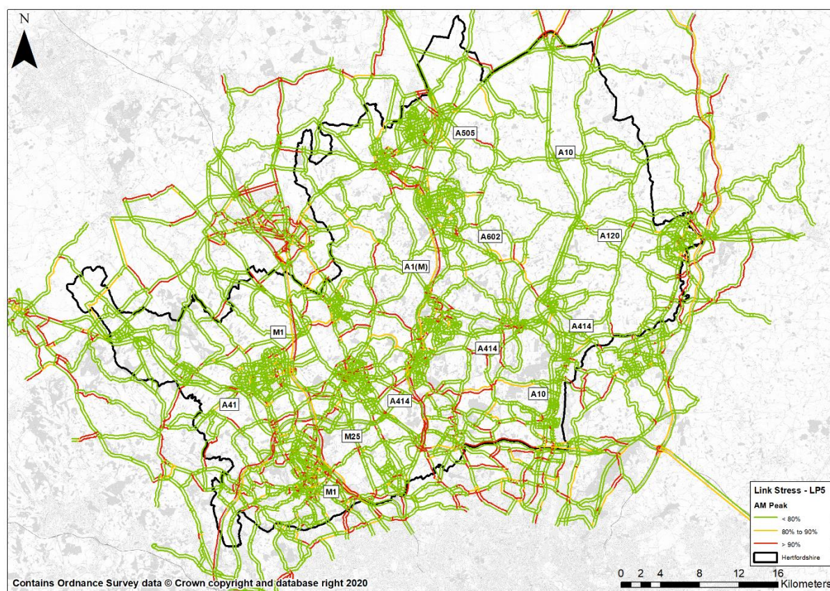
Figure 7-12: COMET 2036 AM Peak Link V/C (All Links)
