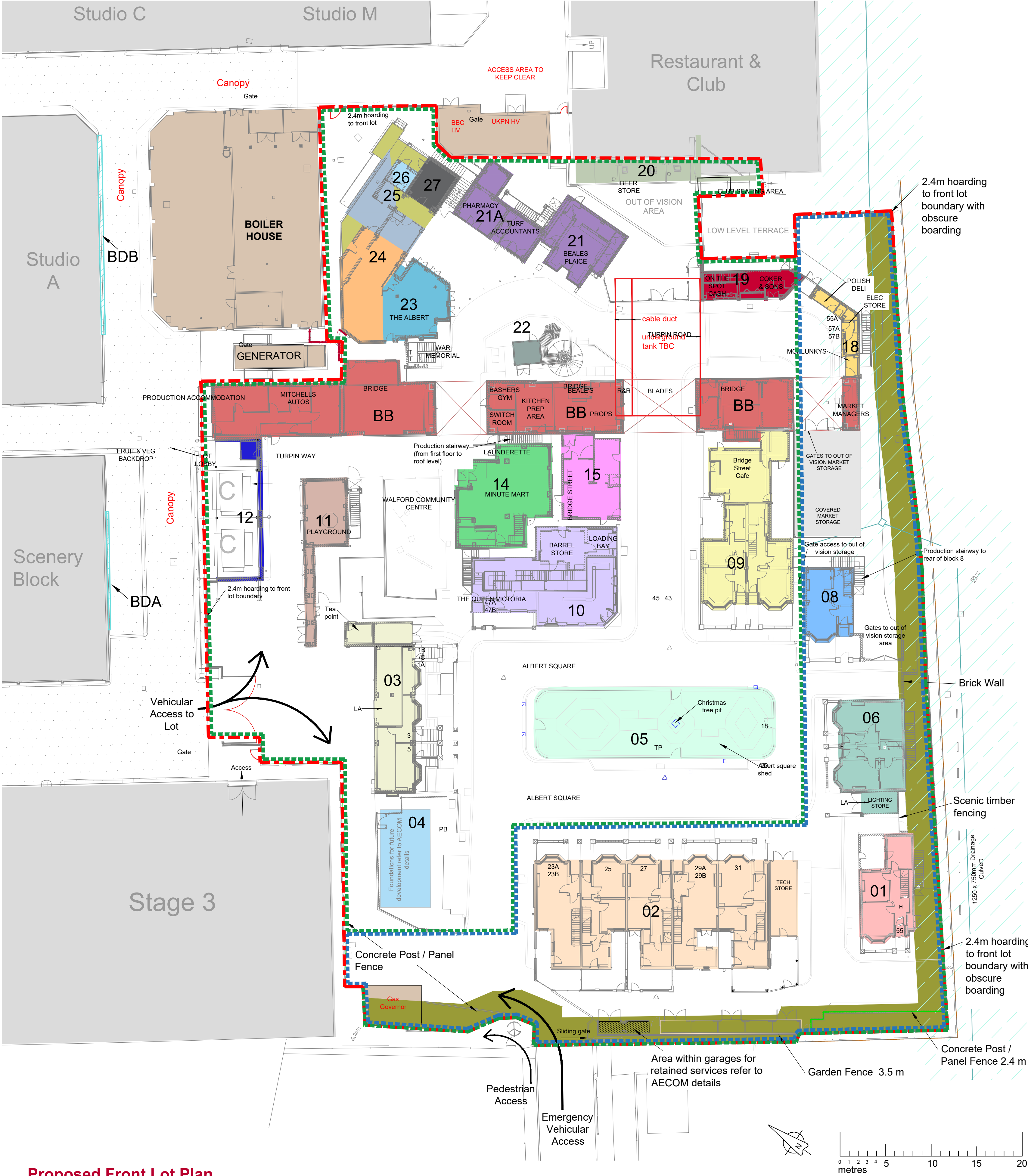
Proposed Front Lot Plan Scale 1:250 @ A1
