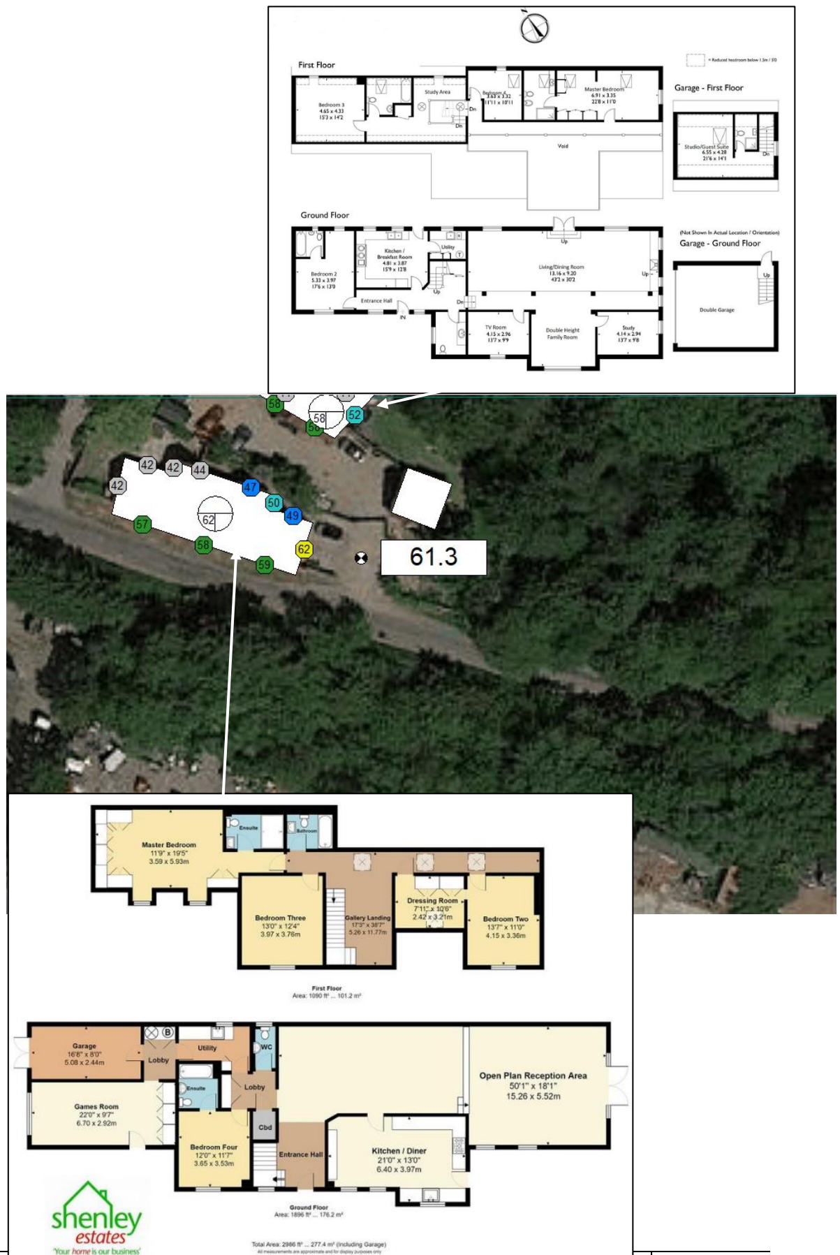
Figure 2 – 1 Hour Commercial Noise Levels Including Character Correction – Existing Dwellings on Mimms Lane & Associated Floor Plans
